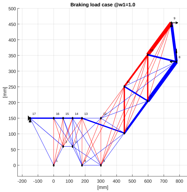
Figure 11: Optimized motorcycle frame for w_1 = 1.0 and w_2 = 0.0
