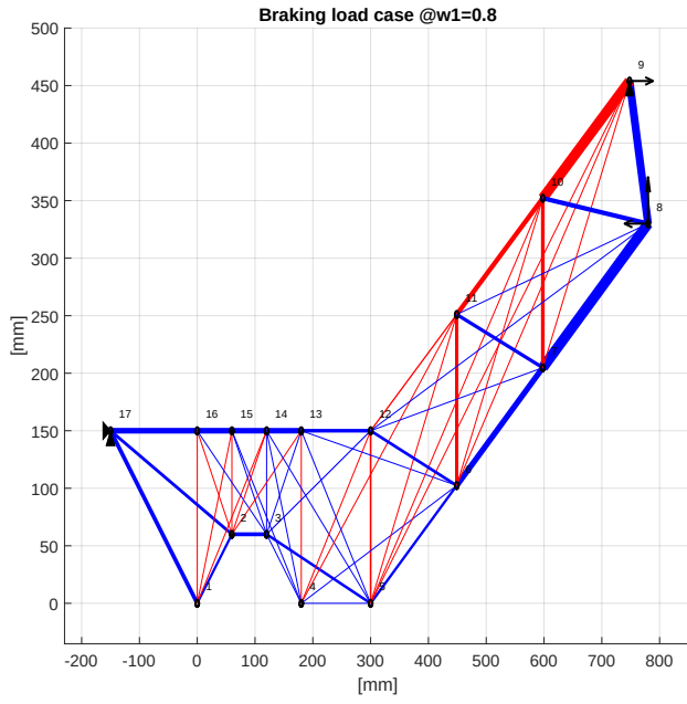
Figure 10: Optimized motorcycle frame for w_1 = 0.8 and w_2 = 0.2
